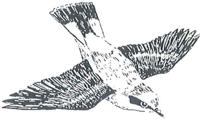
Steinskvett
